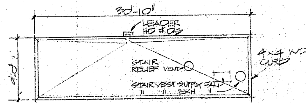
PENTHOUSE ROOF PLAN SC: 1/8" = 1'-0"
