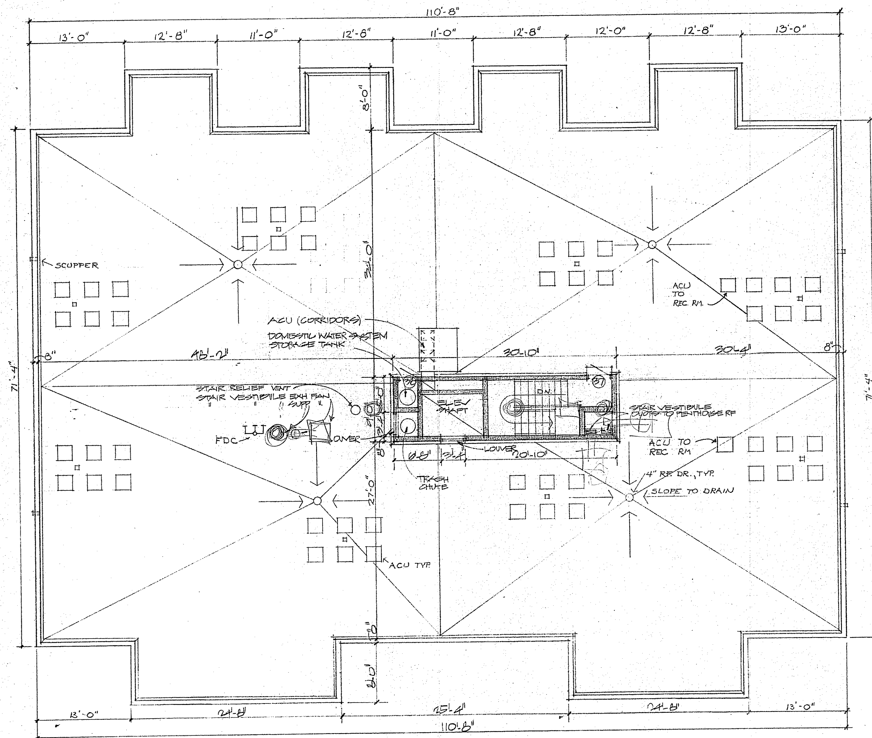
ROOF PLAN SC: 1/8" = 1'-0"
